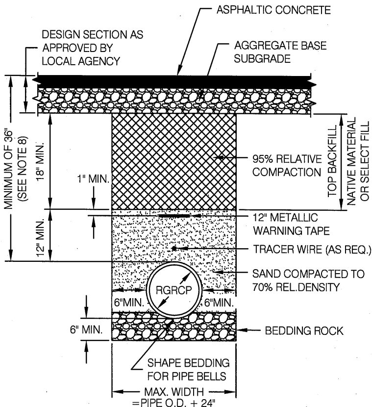
TRENCH IN PROPOSED PAVED PORTIONS
