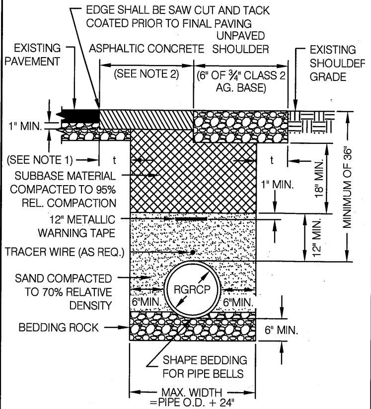
TRENCH IN EXISTING PAVED PORTIONS AND IN UNPAVED SHOULDERS
